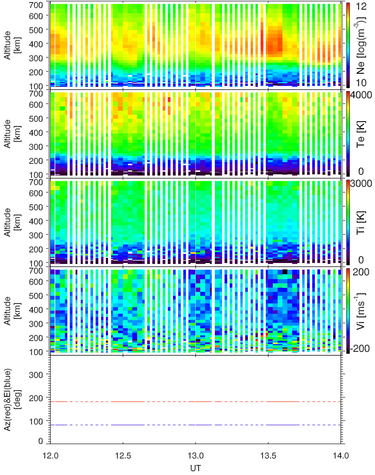
EISCAT 2001-10-09_12_14UT_tau0_120@42m.
