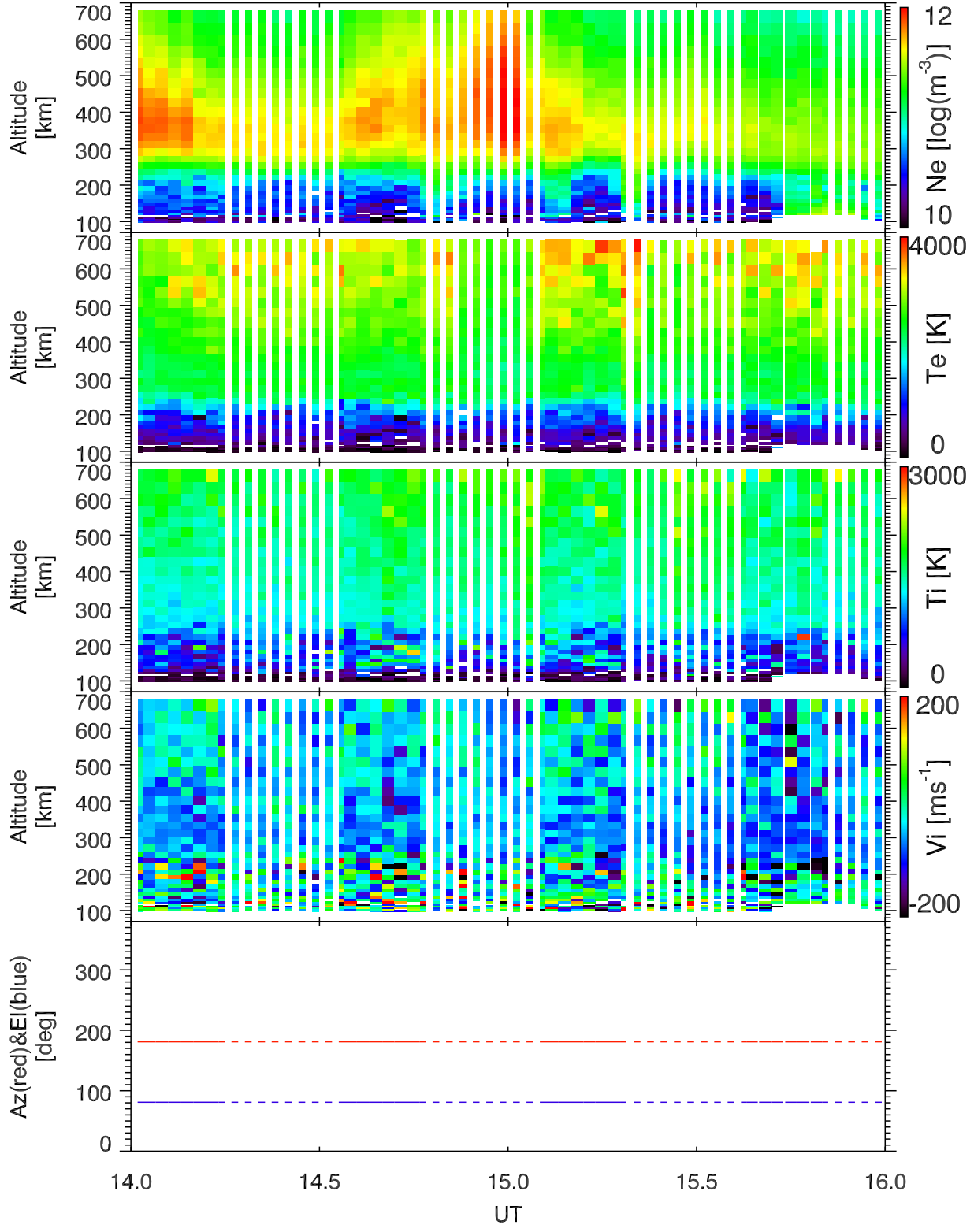
EISCAT 2001-10-09_14_16UT_tau0_120@42m.
