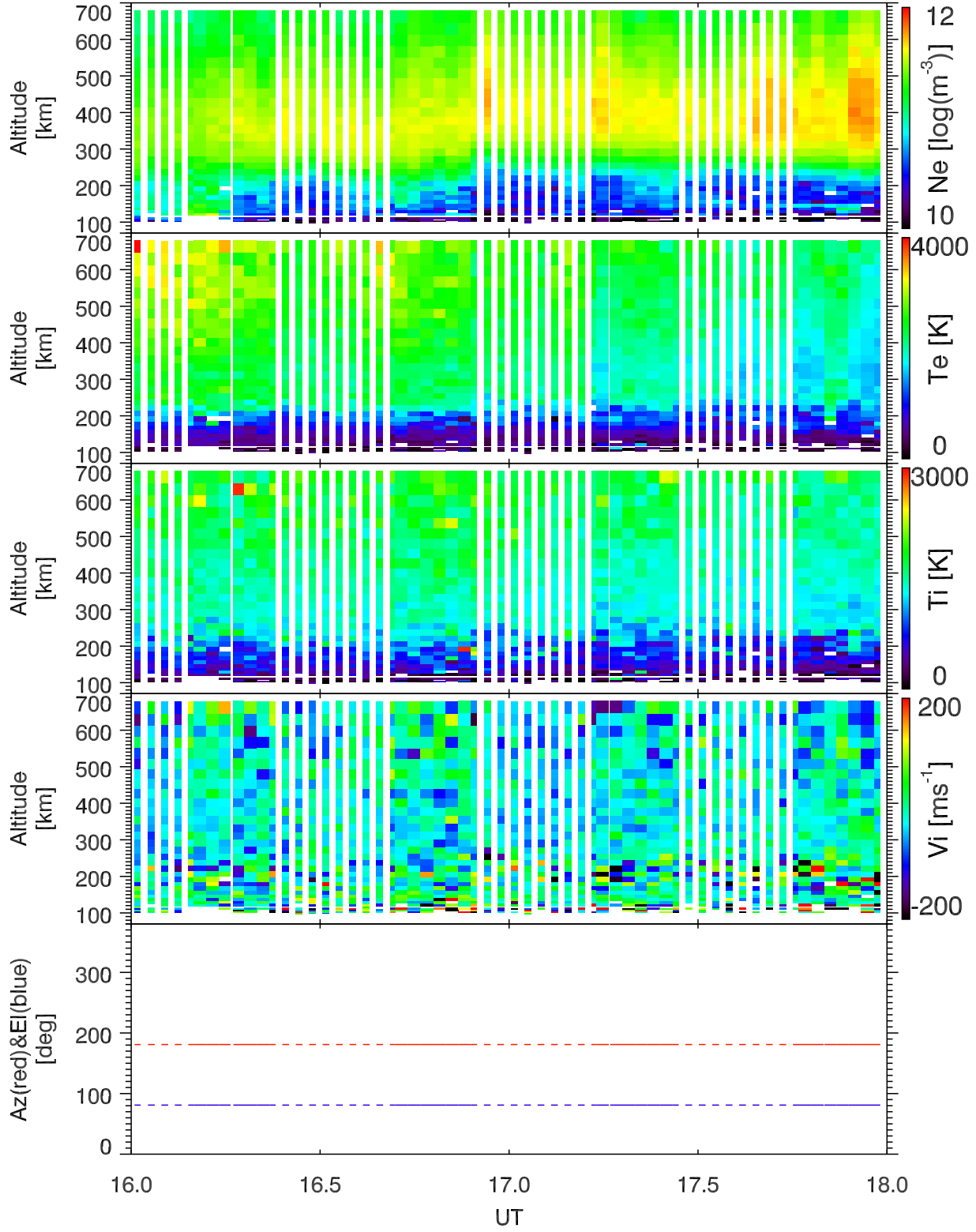
EISCAT 2001-10-09_16_18UT_tau0_120@42m.
