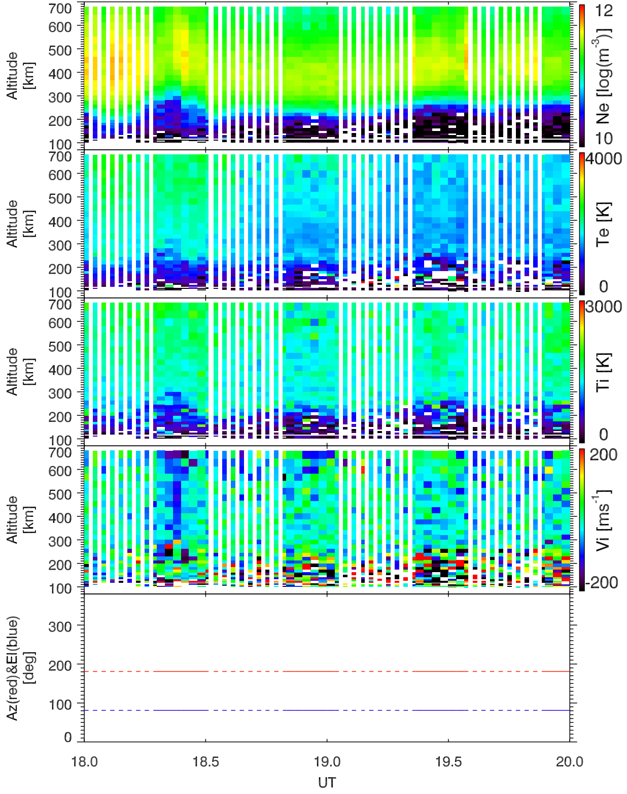
EISCAT 2001-10-09_18_20UT_tau0_120@42m.
