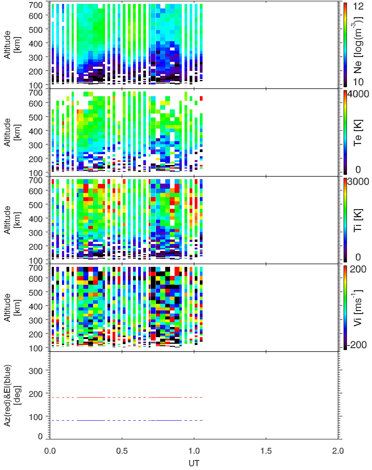
EISCAT 2001-10-10_00_02UT_tau0_120@42m.
