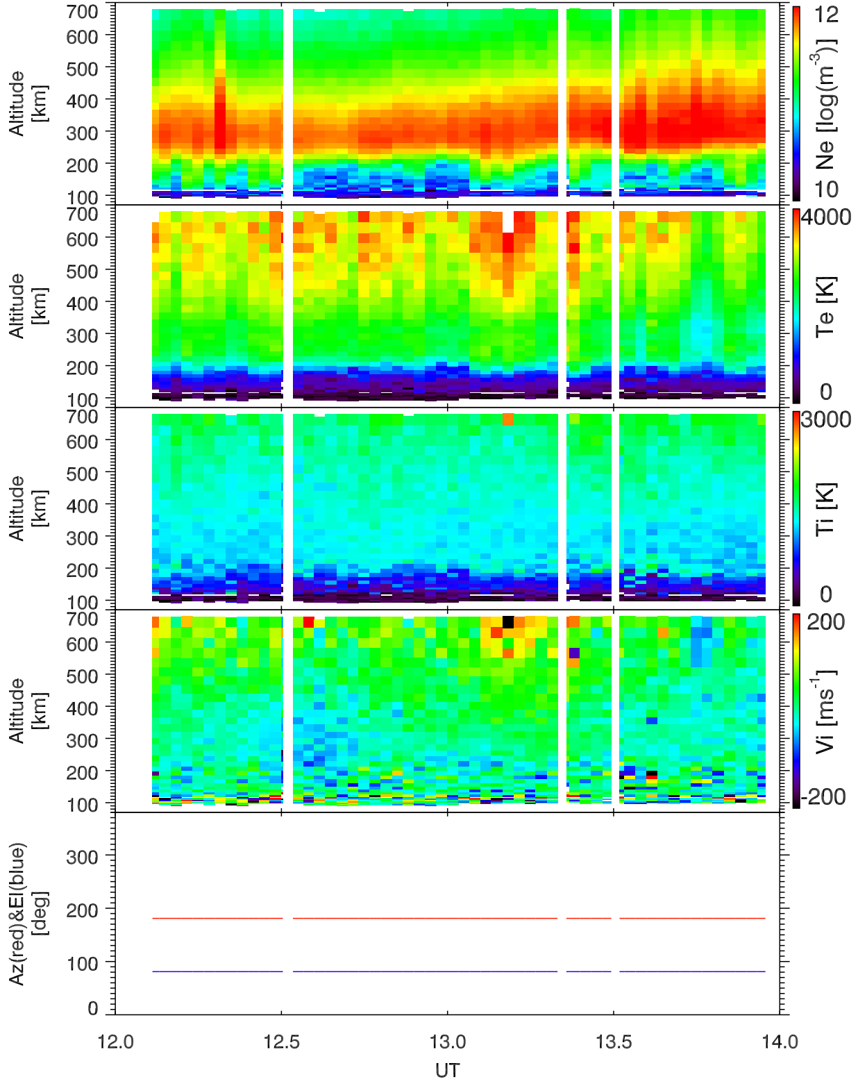
EISCAT 2001-10-16_12_14UT_tau0_120@42m.
