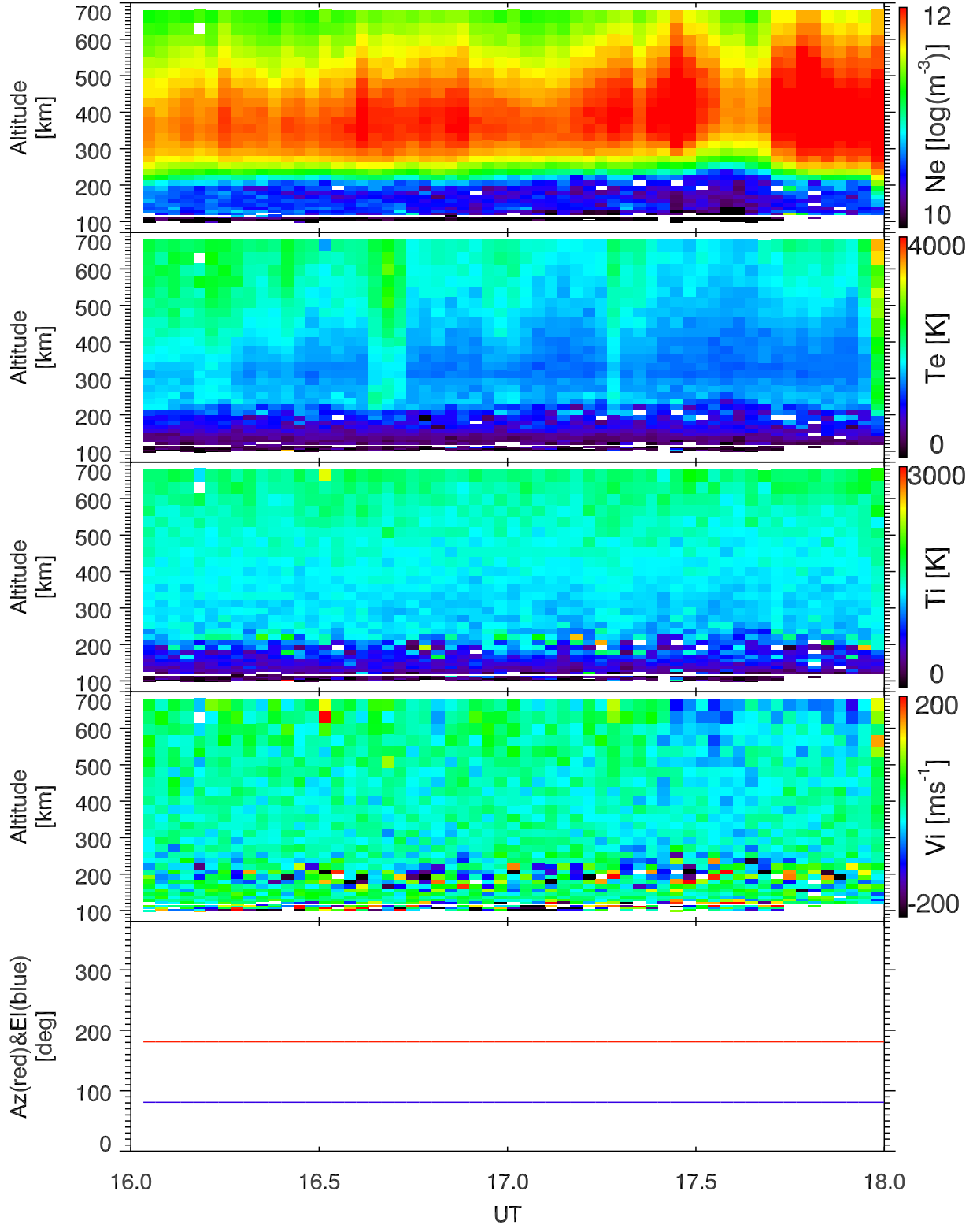
EISCAT 2001-10-16_16_18UT_tau0_120@42m.
