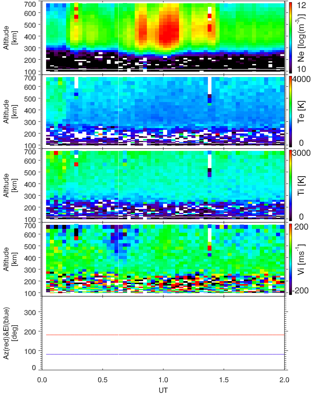
EISCAT 2001-10-17_00_02UT_tau0_120@42m.
