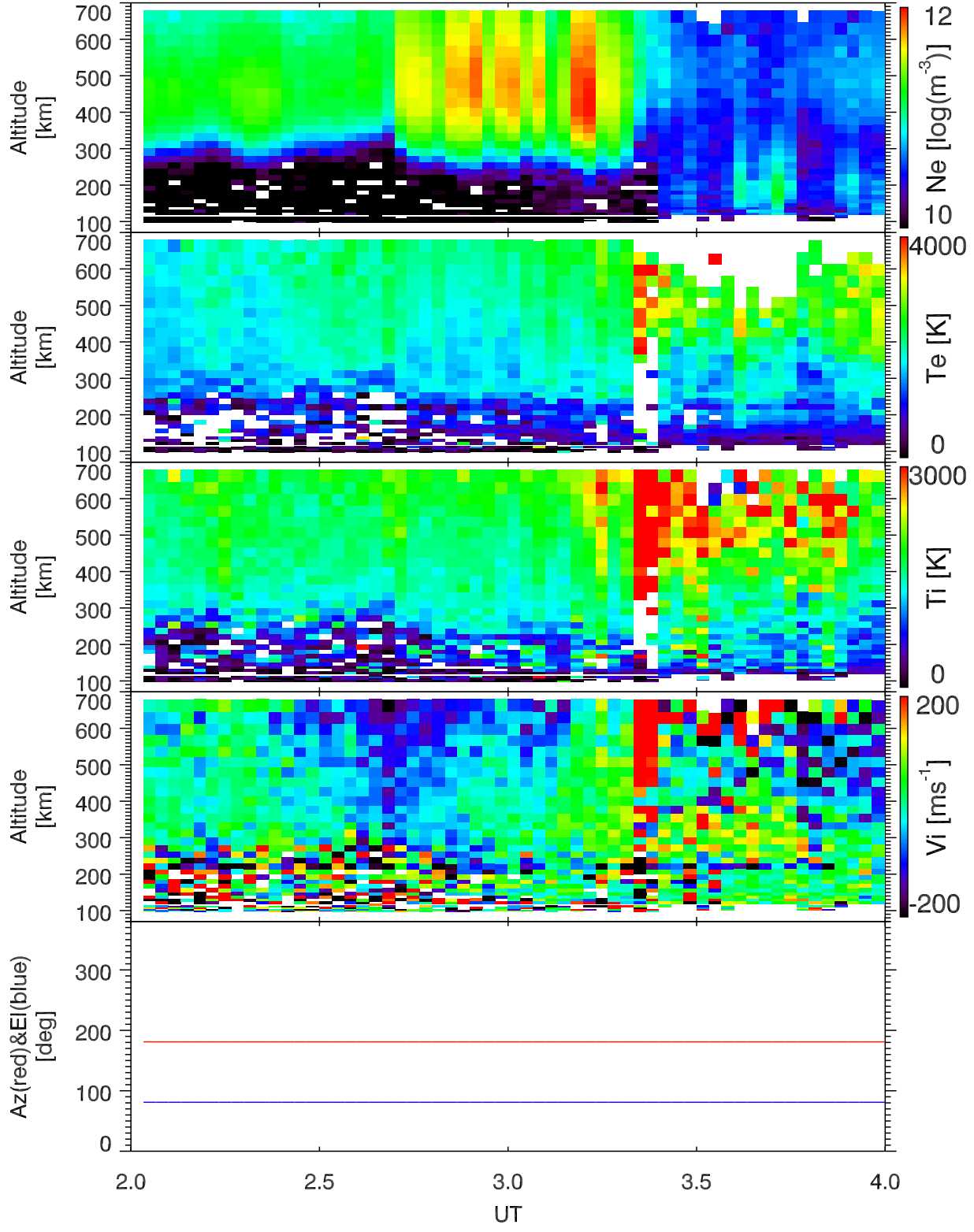
EISCAT 2001-10-17_02_04UT_tau0_120@42m.
