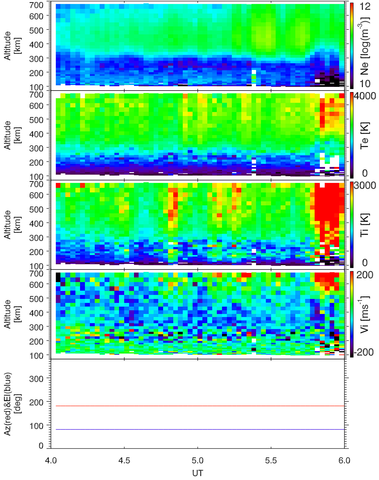
EISCAT 2001-10-17_04_06UT_tau0_120@42m.
