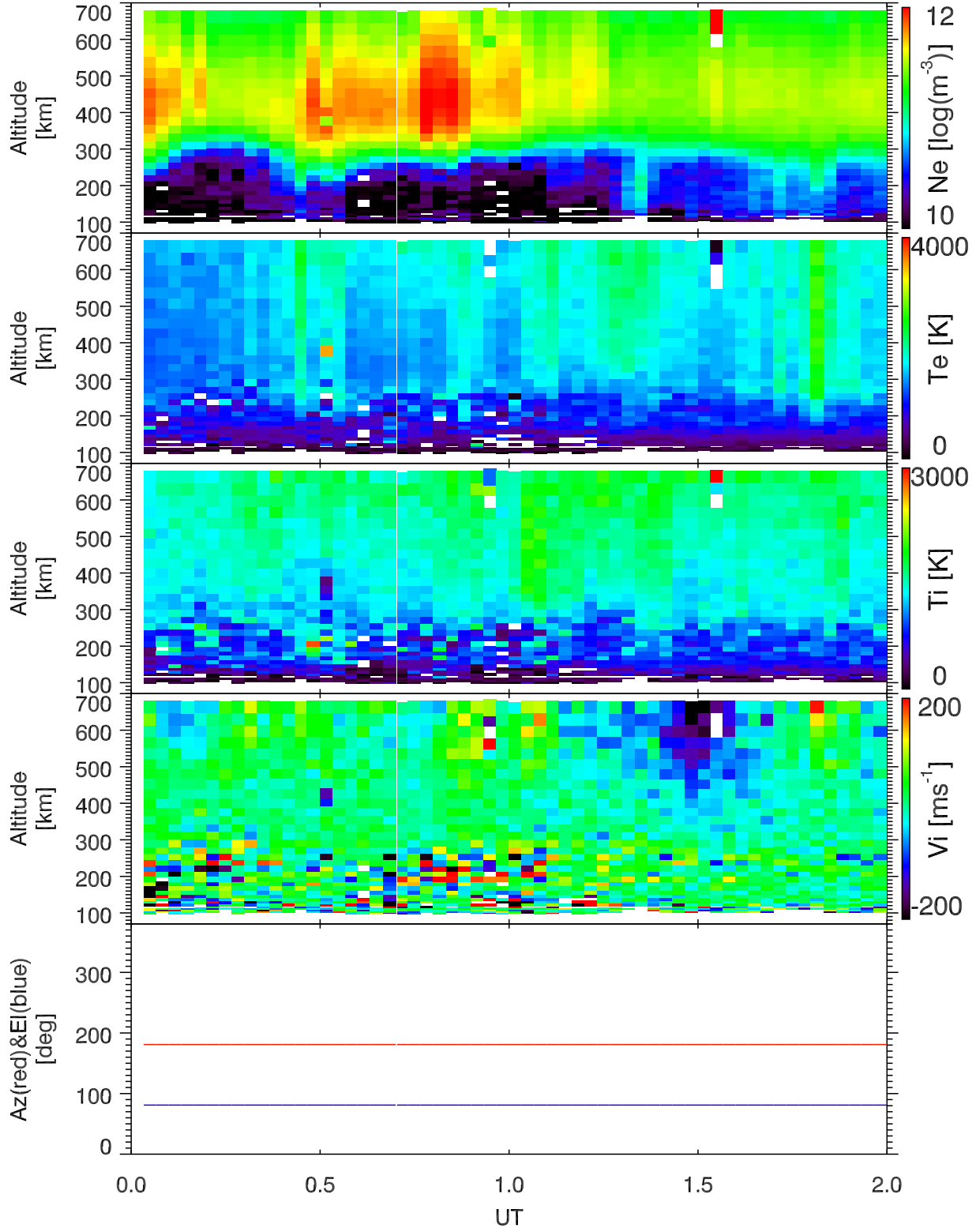
EISCAT 2001-10-18_00_02UT_tau0_120@42m.
