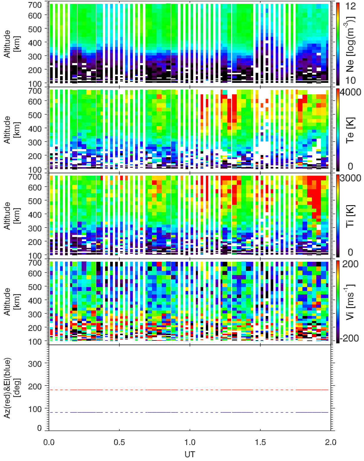
EISCAT 2001-10-20_00_02UT_tau0_120@42m.
