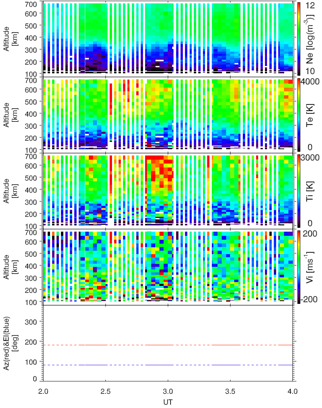
EISCAT 2001-10-20_02_04UT_tau0_120@42m.
