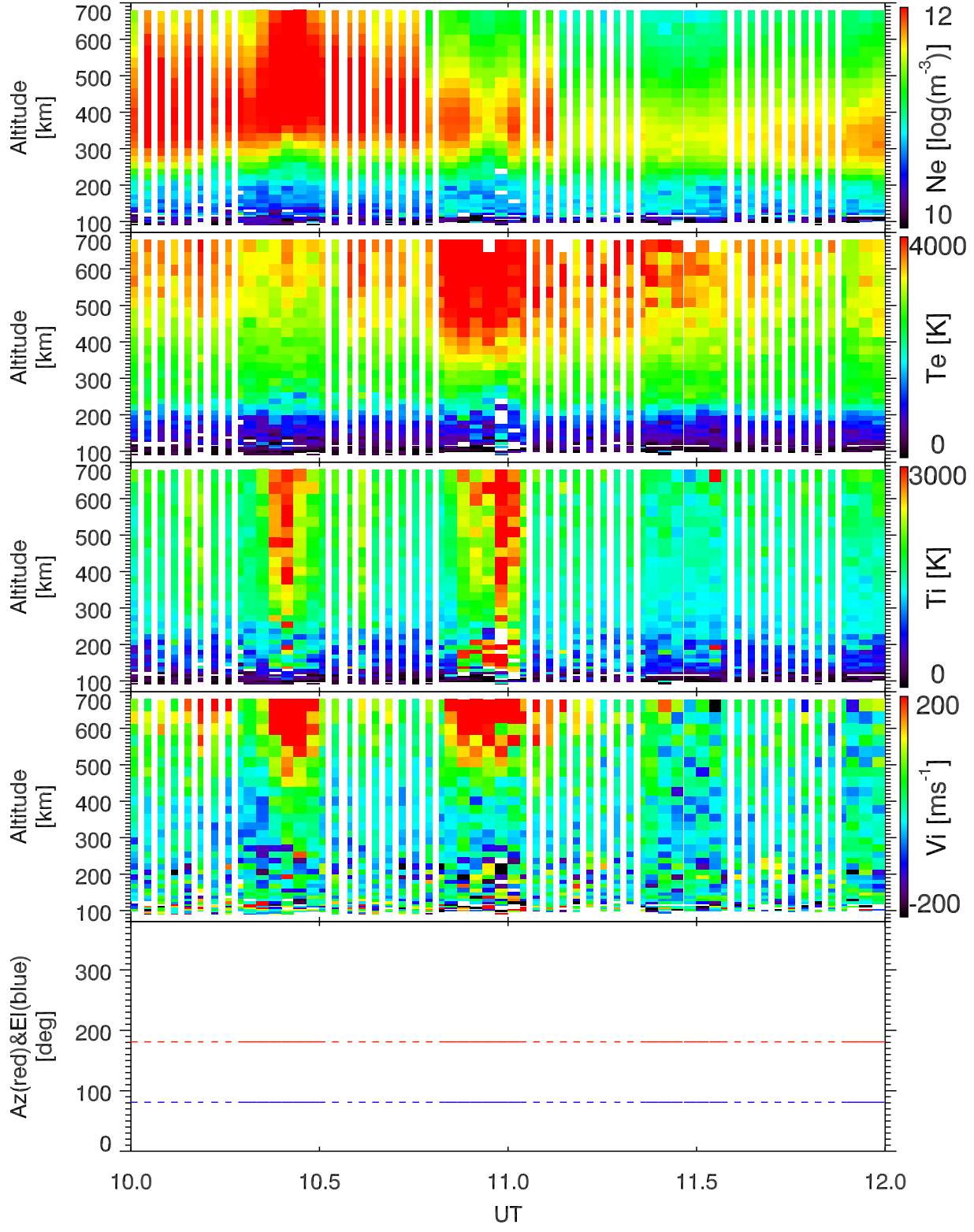
EISCAT 2001-10-20_10_12UT_tau0_120@42m.
