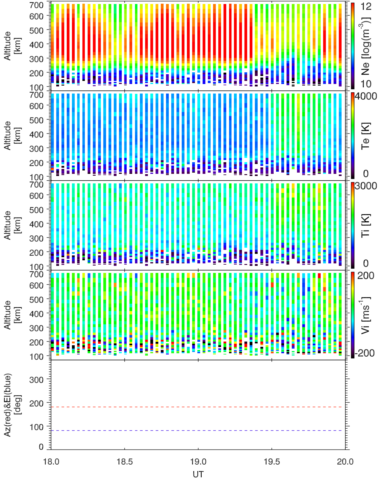
EISCAT 2001-10-27_18_20UT_tau0_ant@42m.
