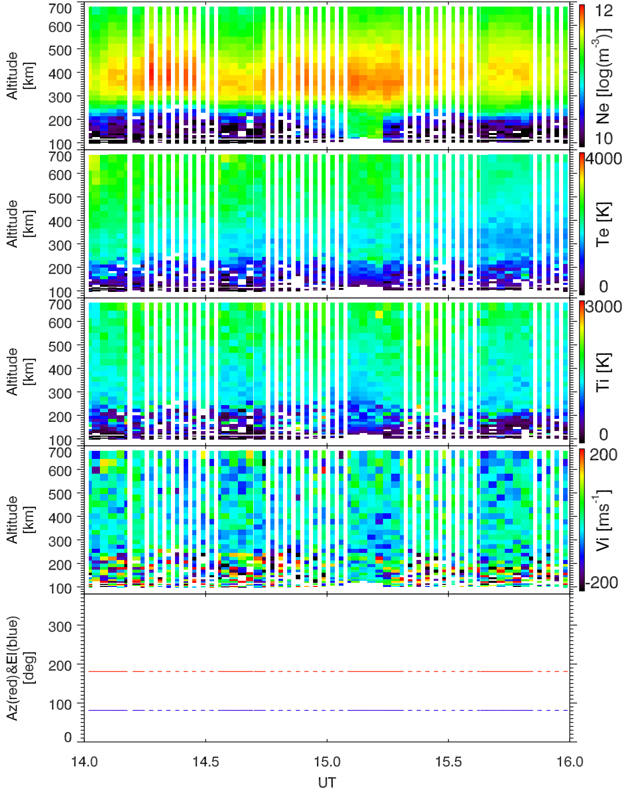
EISCAT 2001-10-29_14_16UT_tau0_120@42m.
