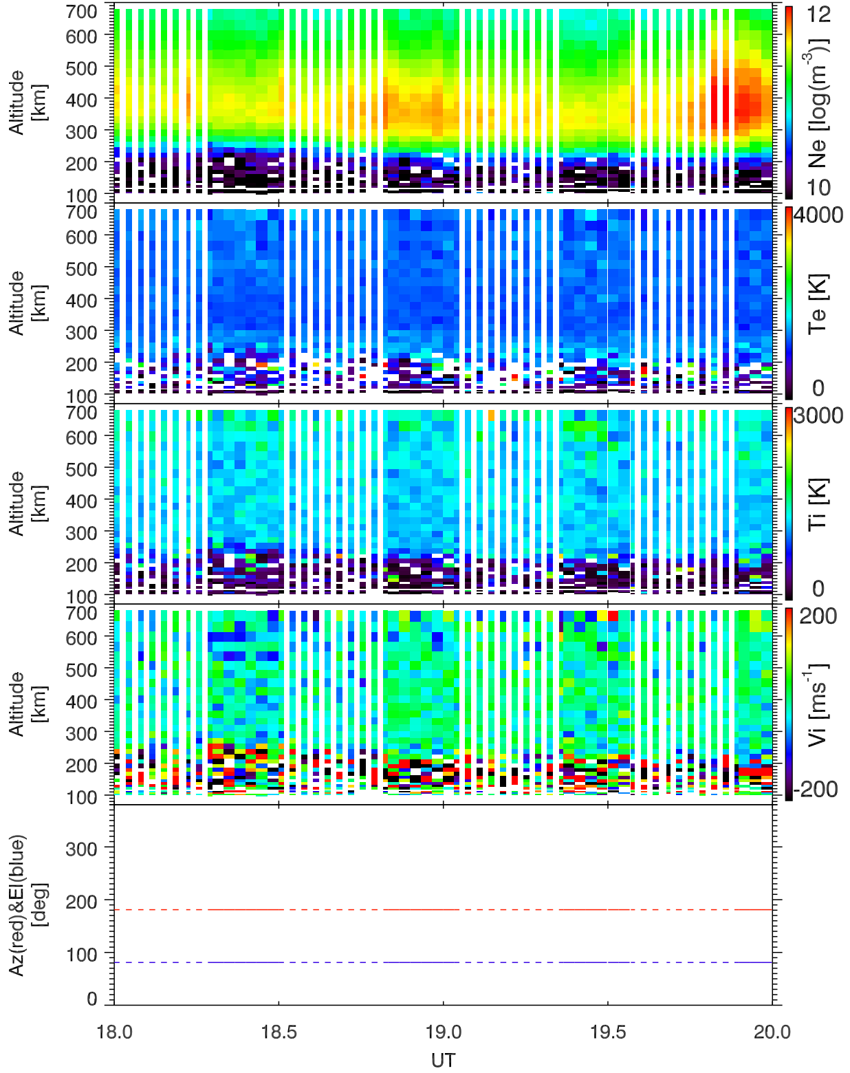
EISCAT 2001-10-30_18_20UT_tau0_120@42m.
