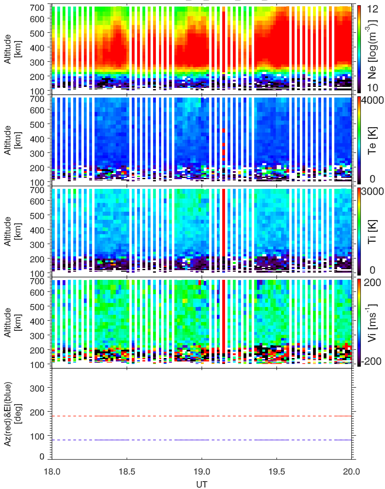
EISCAT 2001-11-03_18_20UT_tau0_all@42m.
