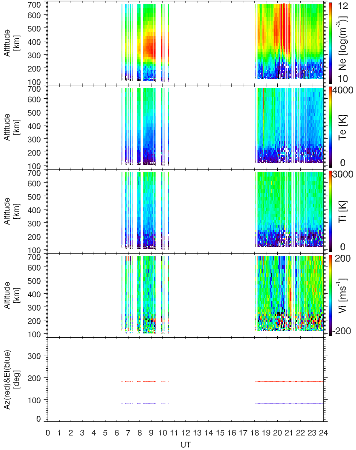
EISCAT 2001-11-05_00_24UT_tau0_120@42m.
