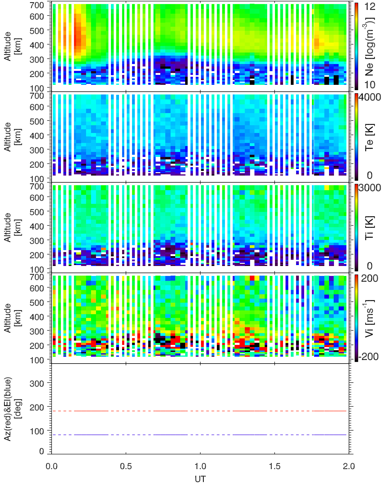
EISCAT 2001-11-06_00_02UT_tau0_120@42m.
