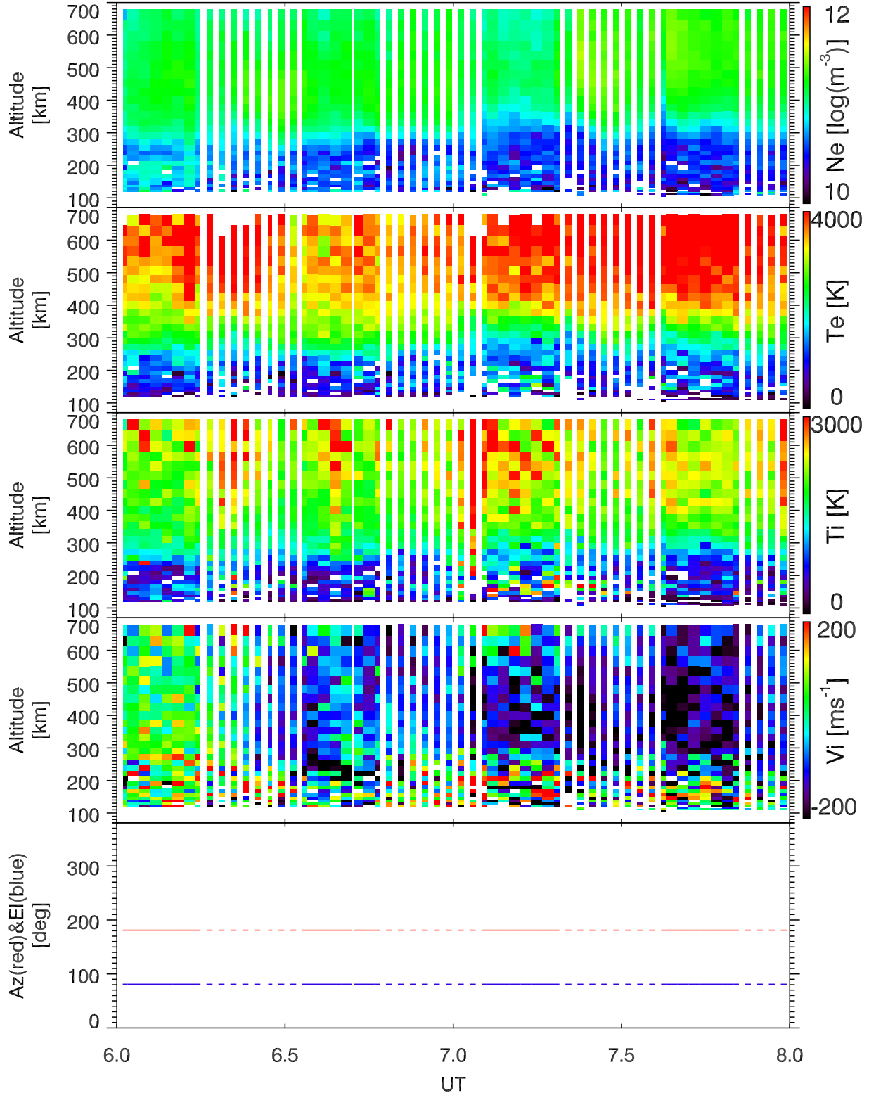
EISCAT 2001-11-06_06_08UT_tau0_120@42m.
