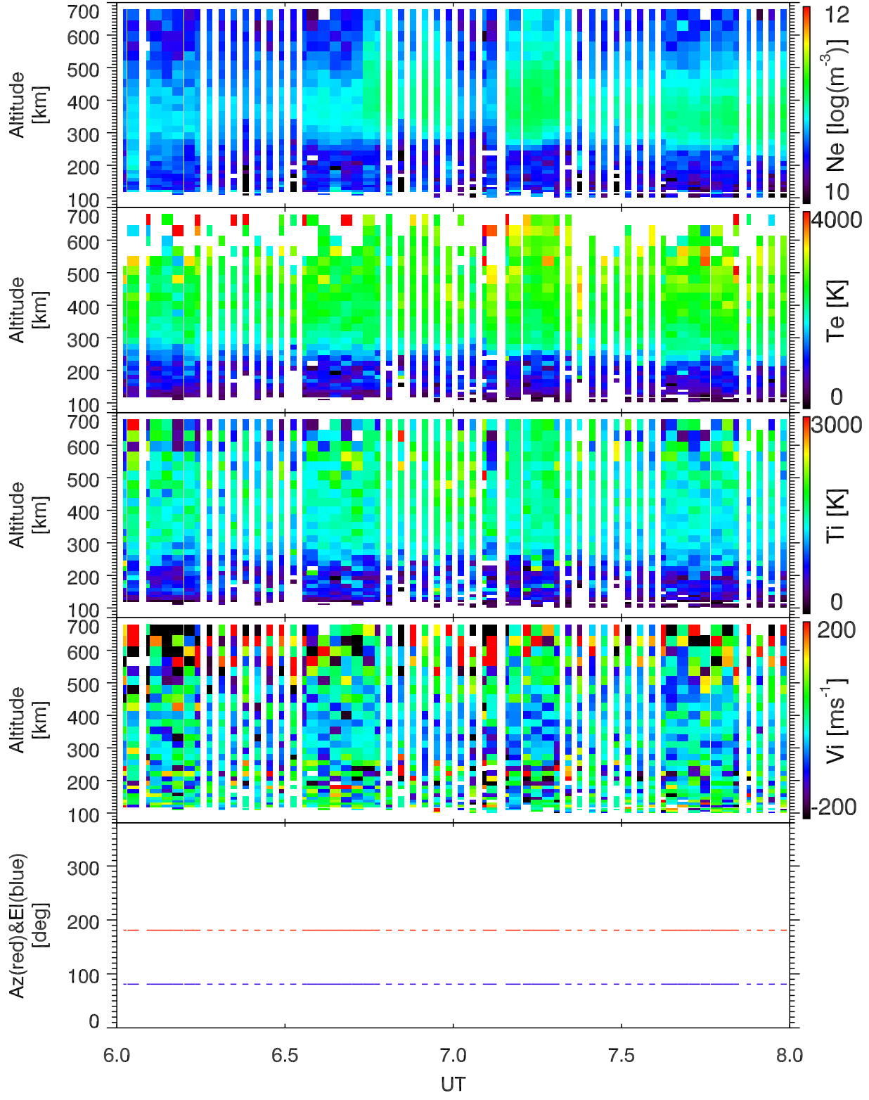
EISCAT 2001-11-07_06_08UT_tau0_120@42m.
