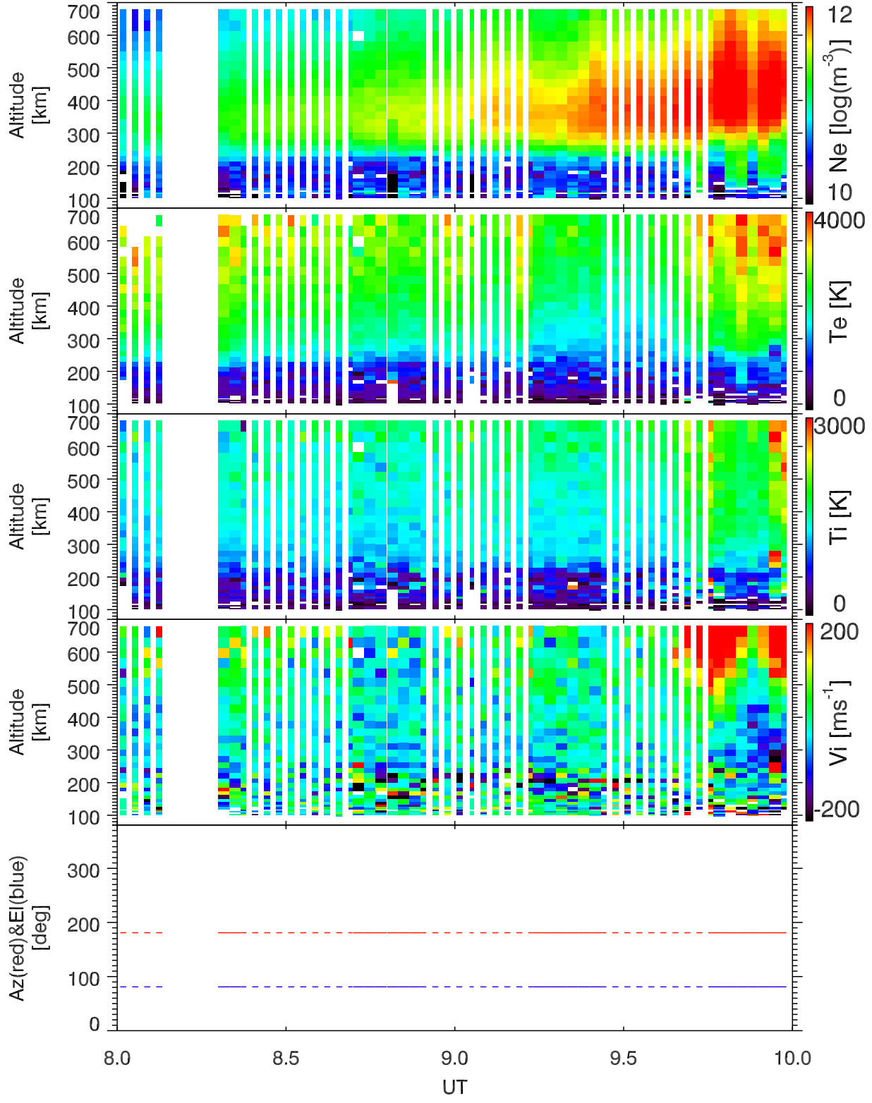
EISCAT 2001-11-07_08_10UT_tau0_120@42m.
