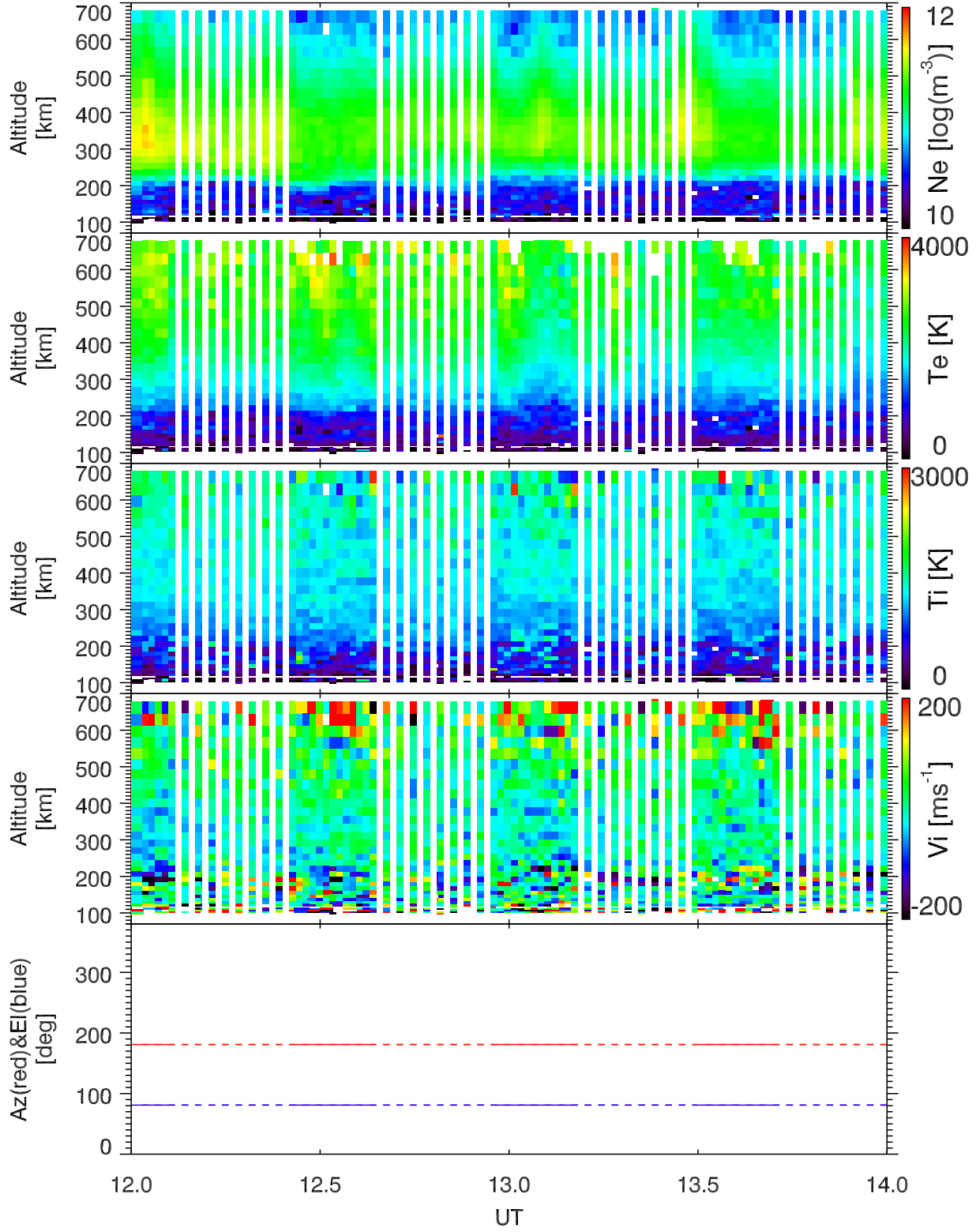
EISCAT 2001-11-11_12_14UT_tau0_all@42m.
