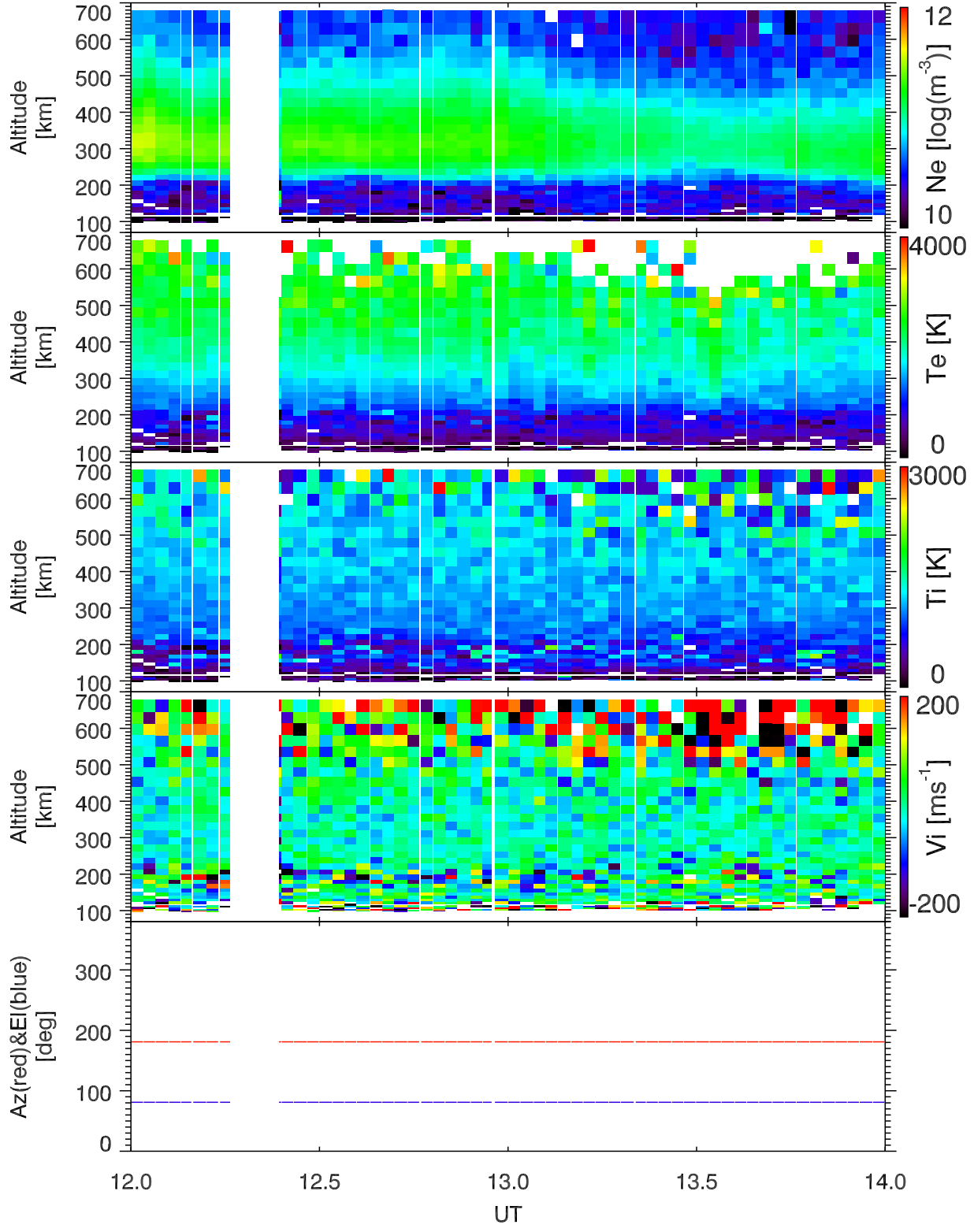
EISCAT 2001-11-13_12_14UT_tau0_120@42m.
