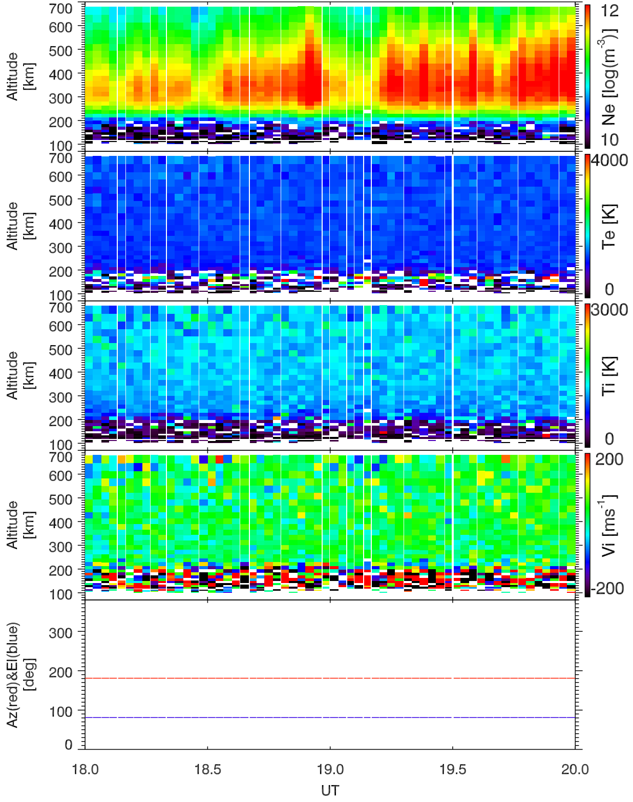
EISCAT 2001-11-13_18_20UT_tau0_120@42m.
