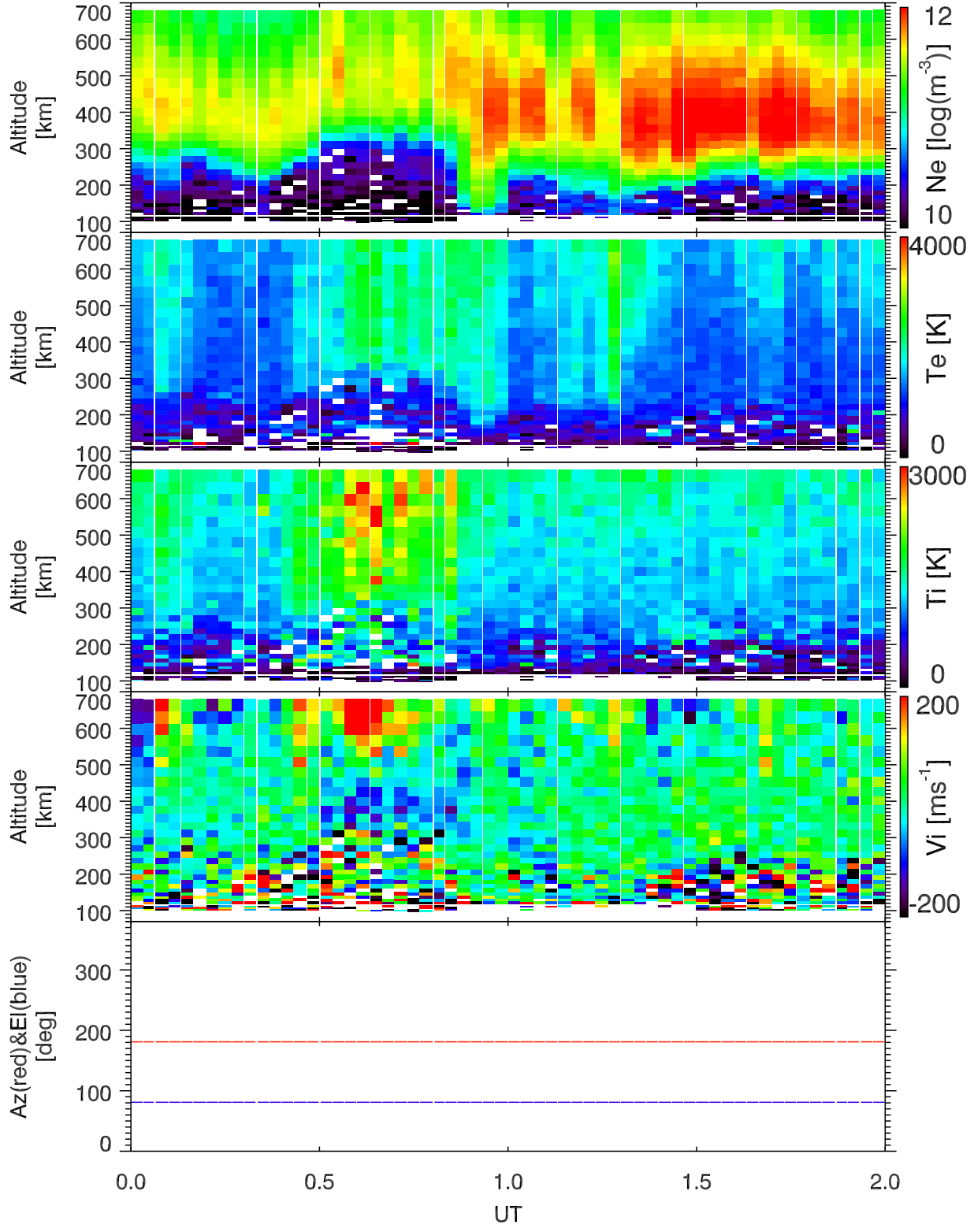
EISCAT 2001-11-14_00_02UT_tau0_120@42m.
