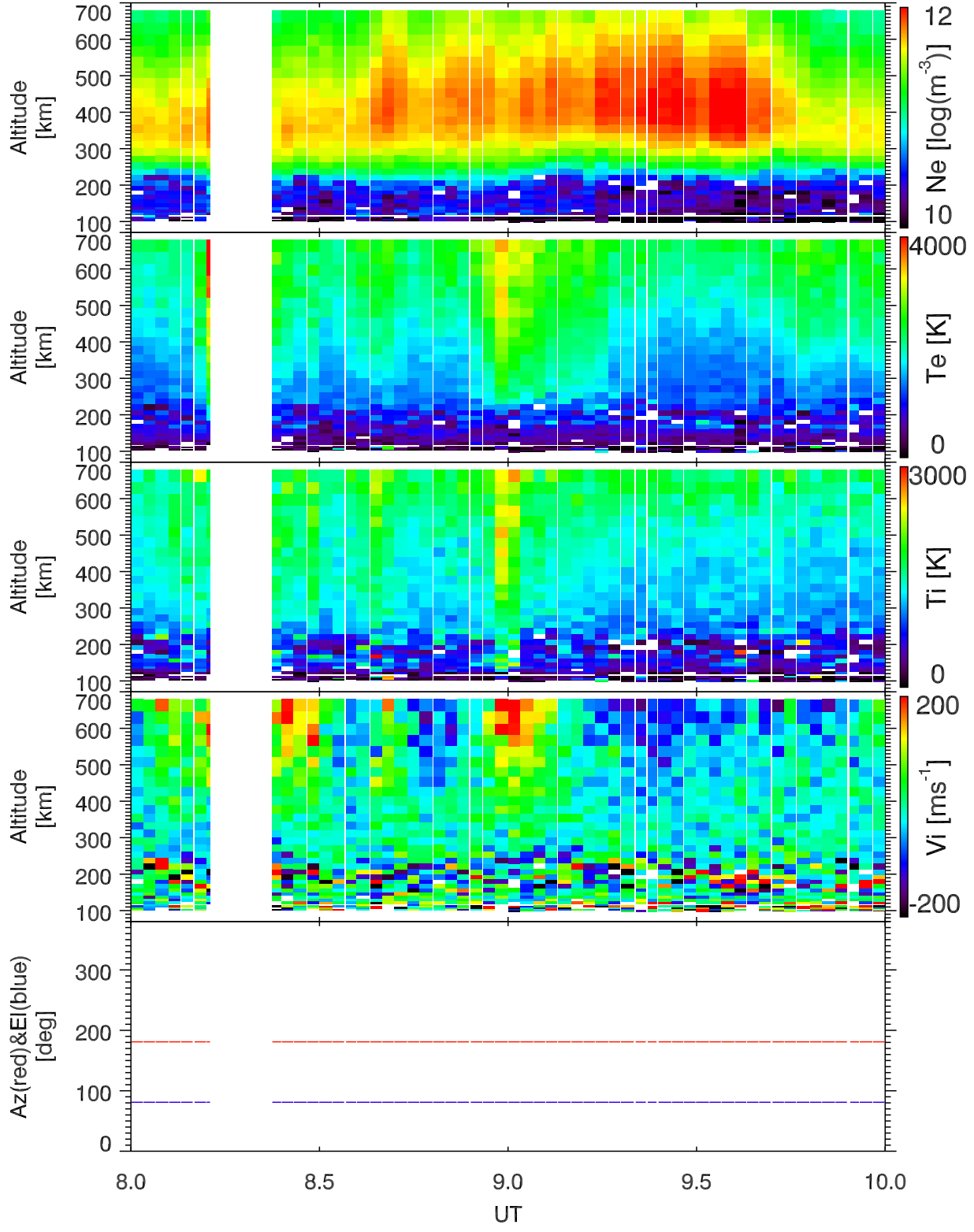
EISCAT 2001-11-14_08_10UT_tau0_120@42m.
