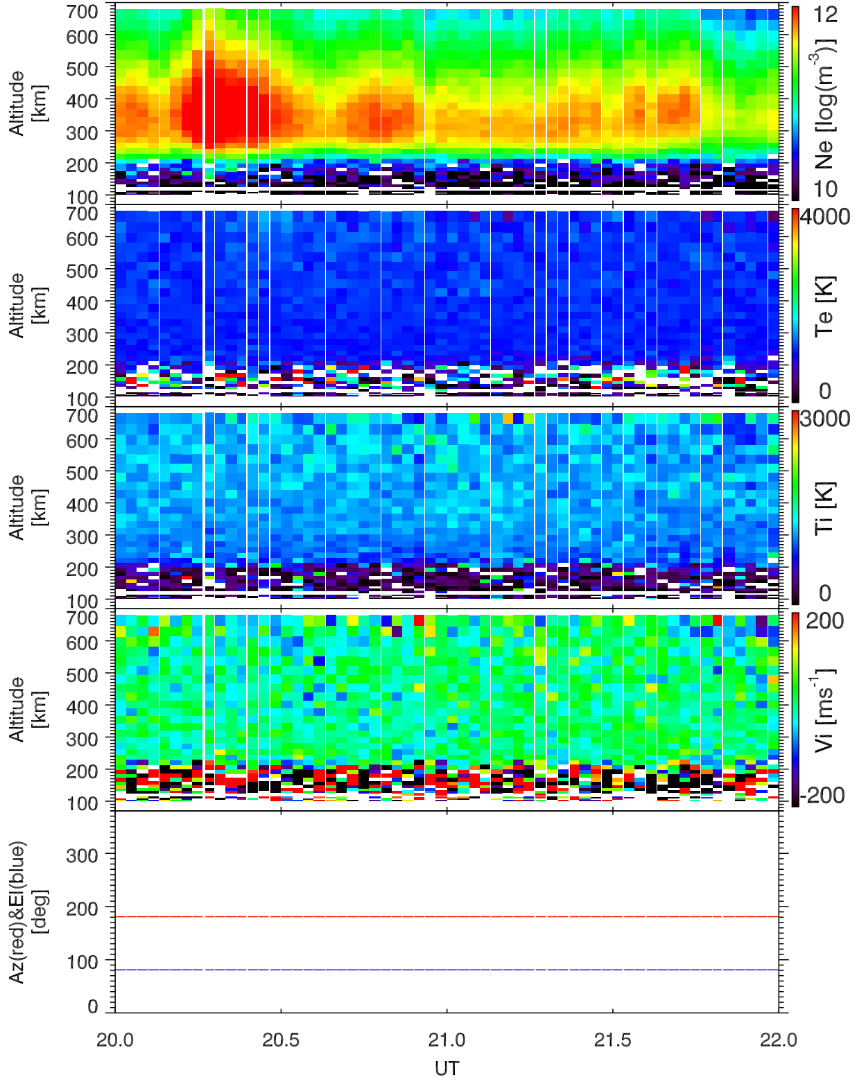
EISCAT 2001-11-14_20_22UT_tau0_120@42m.
