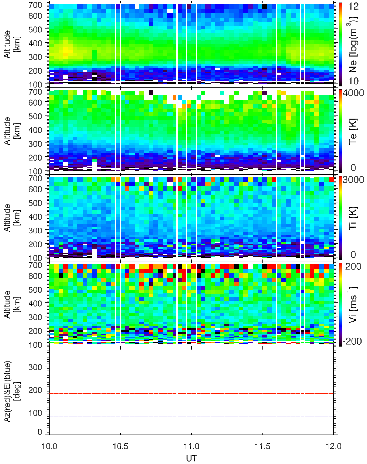
EISCAT 2001-11-15_10_12UT_tau0_all@42m.
