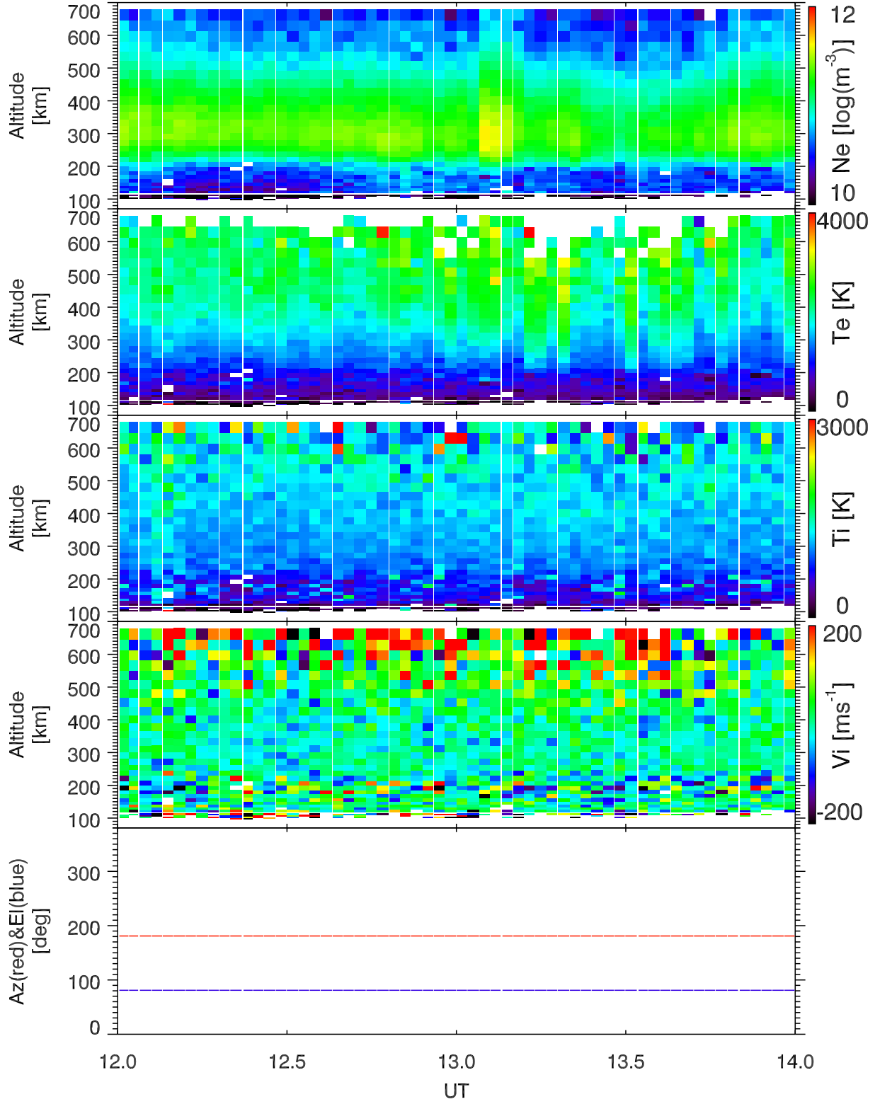
EISCAT 2001-11-15_12_14UT_tau0_all@42m.
