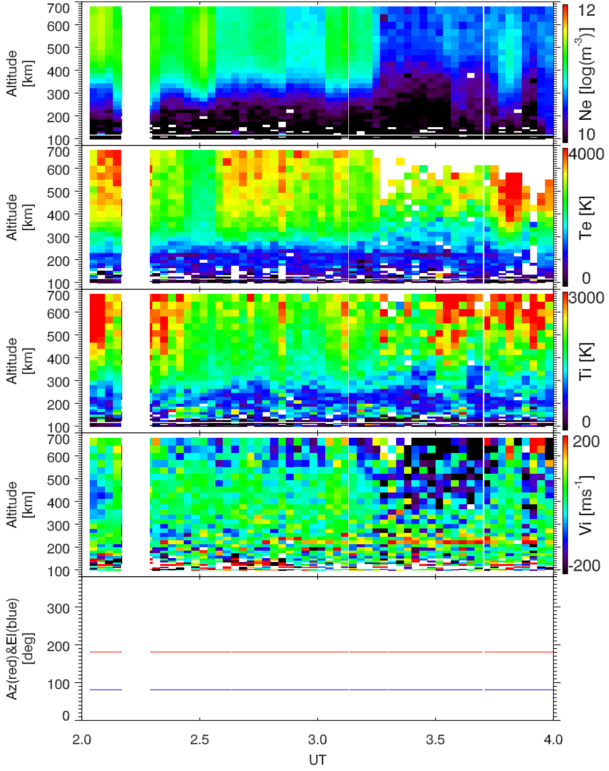
EISCAT 2001-11-16_02_04UT_tau0_120@42m.
