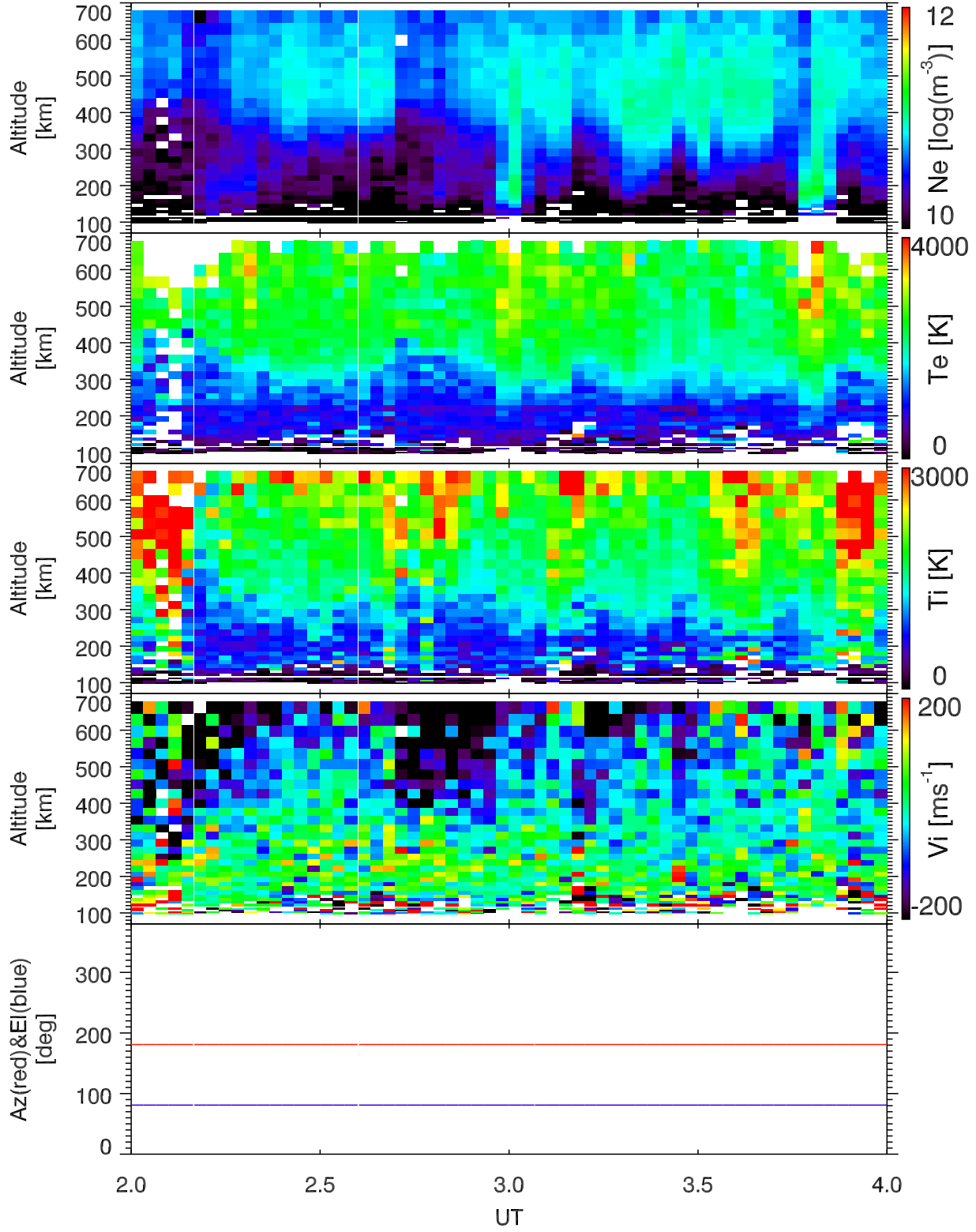
EISCAT 2001-11-18_02_04UT_tau0_all@42m.
