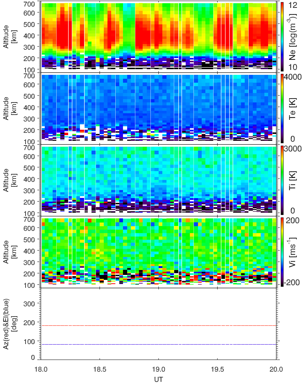
EISCAT 2001-11-18_18_20UT_tau0_all@42m.
