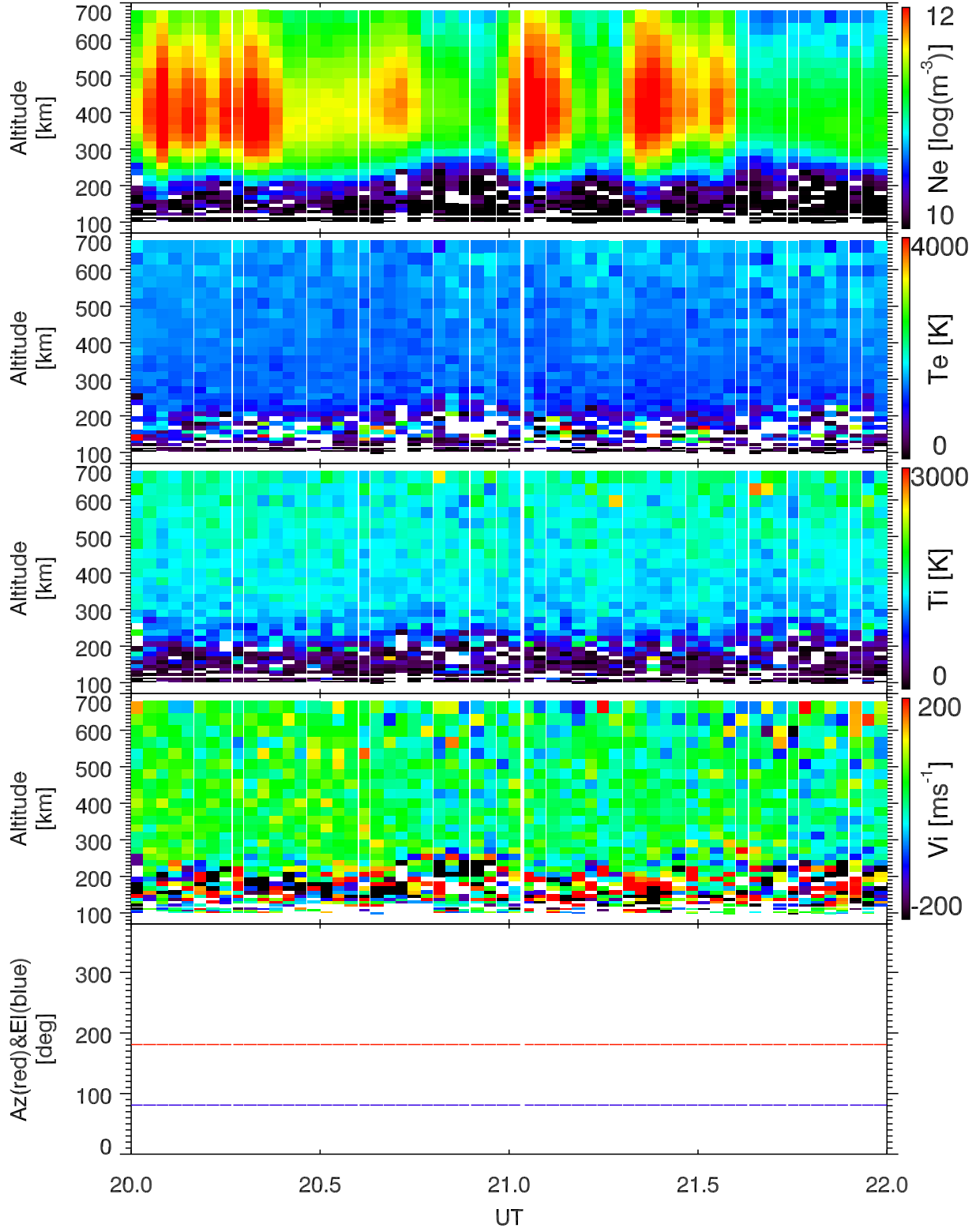
EISCAT 2001-11-18_20_22UT_tau0_all@42m.
