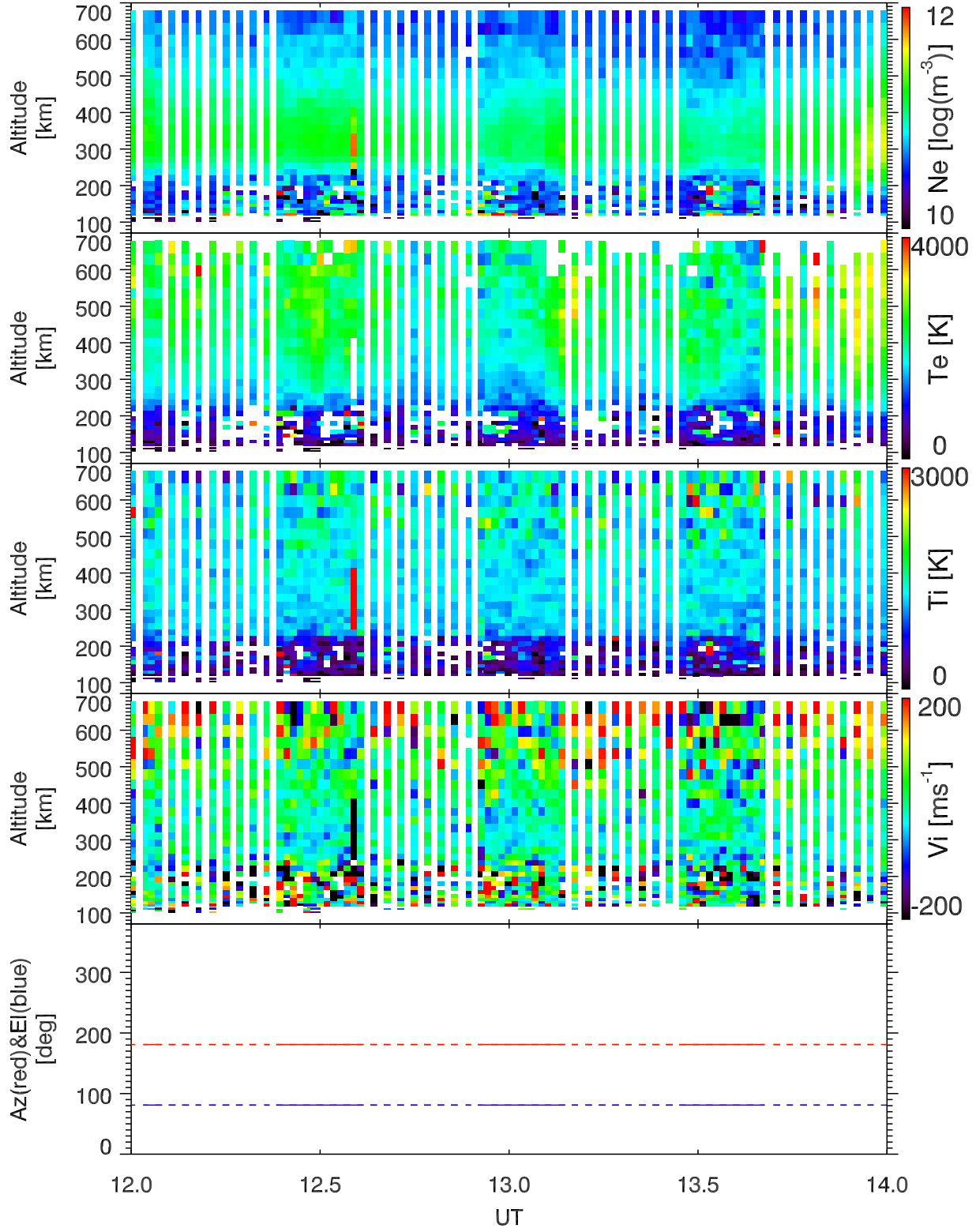
EISCAT 2001-11-20_12_14UT_tau0_all@42m.
