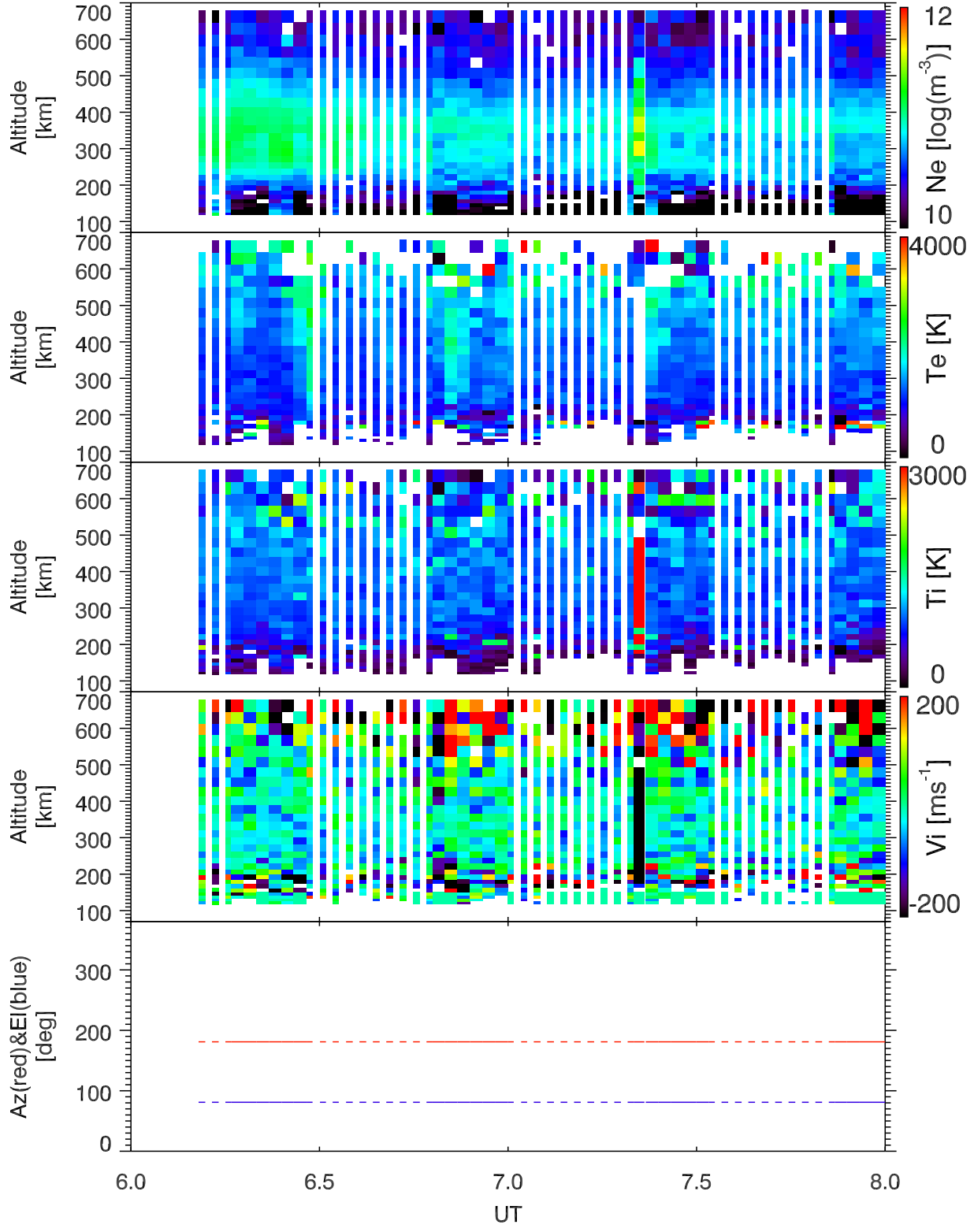
EISCAT 2001-11-27_06_08UT_tau0_120@42m.
