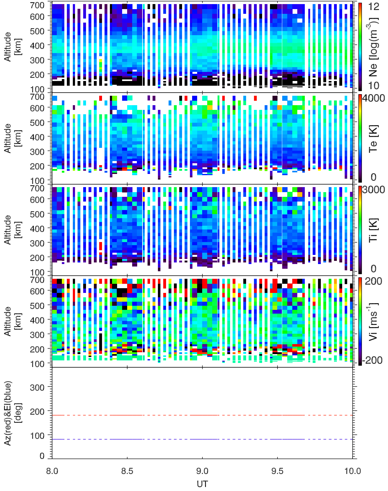
EISCAT 2001-11-27_08_10UT_tau0_120@42m.
