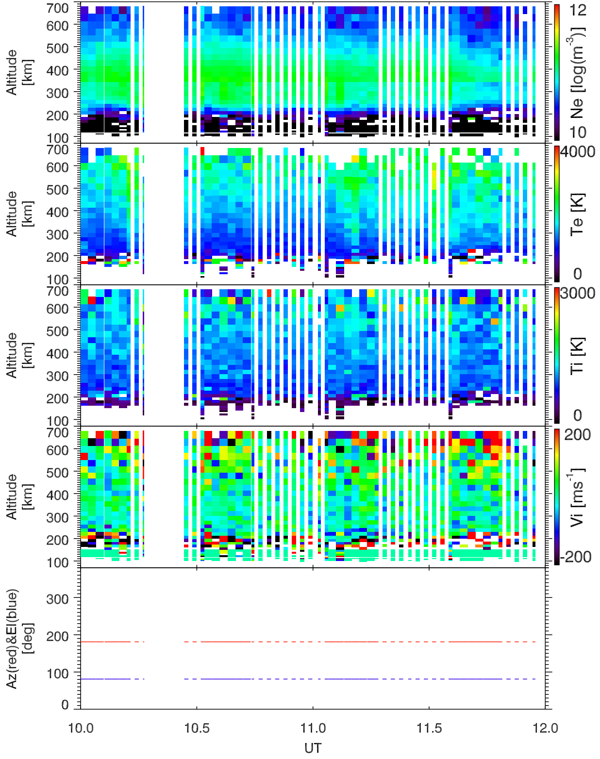
EISCAT 2001-11-27_10_12UT_tau0_120@42m.
