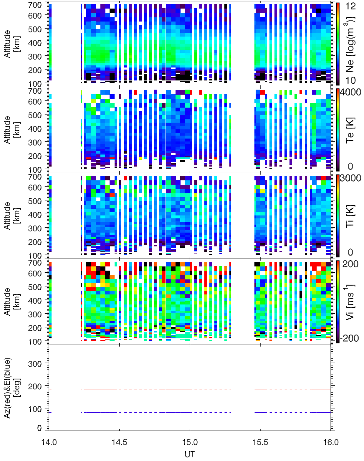
EISCAT 2001-11-27_14_16UT_tau0_120@42m.
