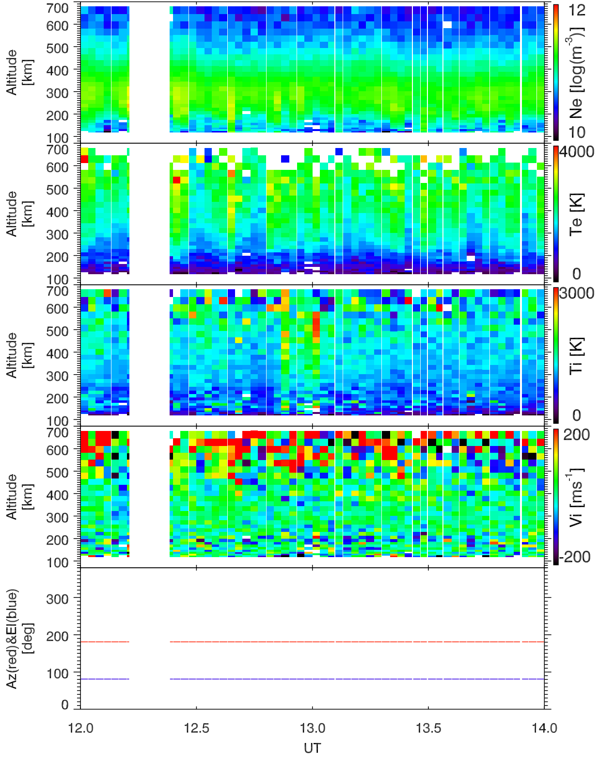
EISCAT 2001-12-11_12_14UT_tau0_120@42m.
