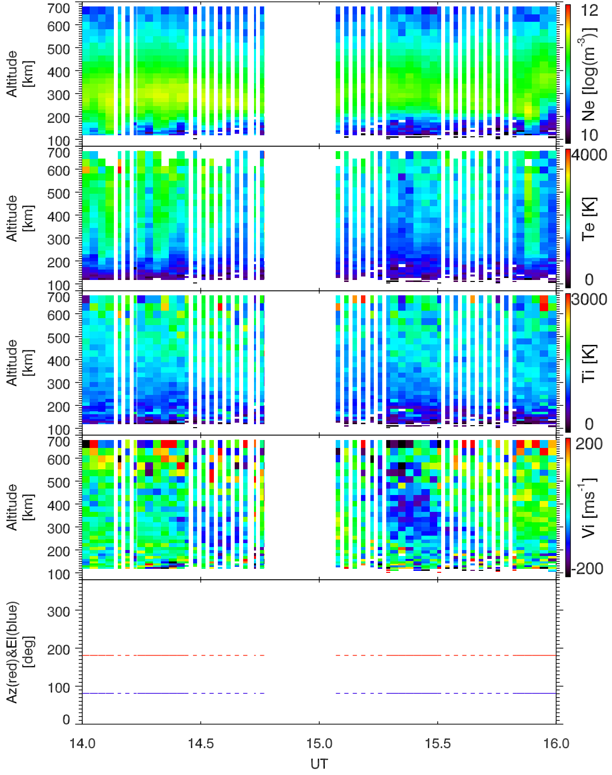
EISCAT 2001-12-11_14_16UT_tau0_120@42m.
