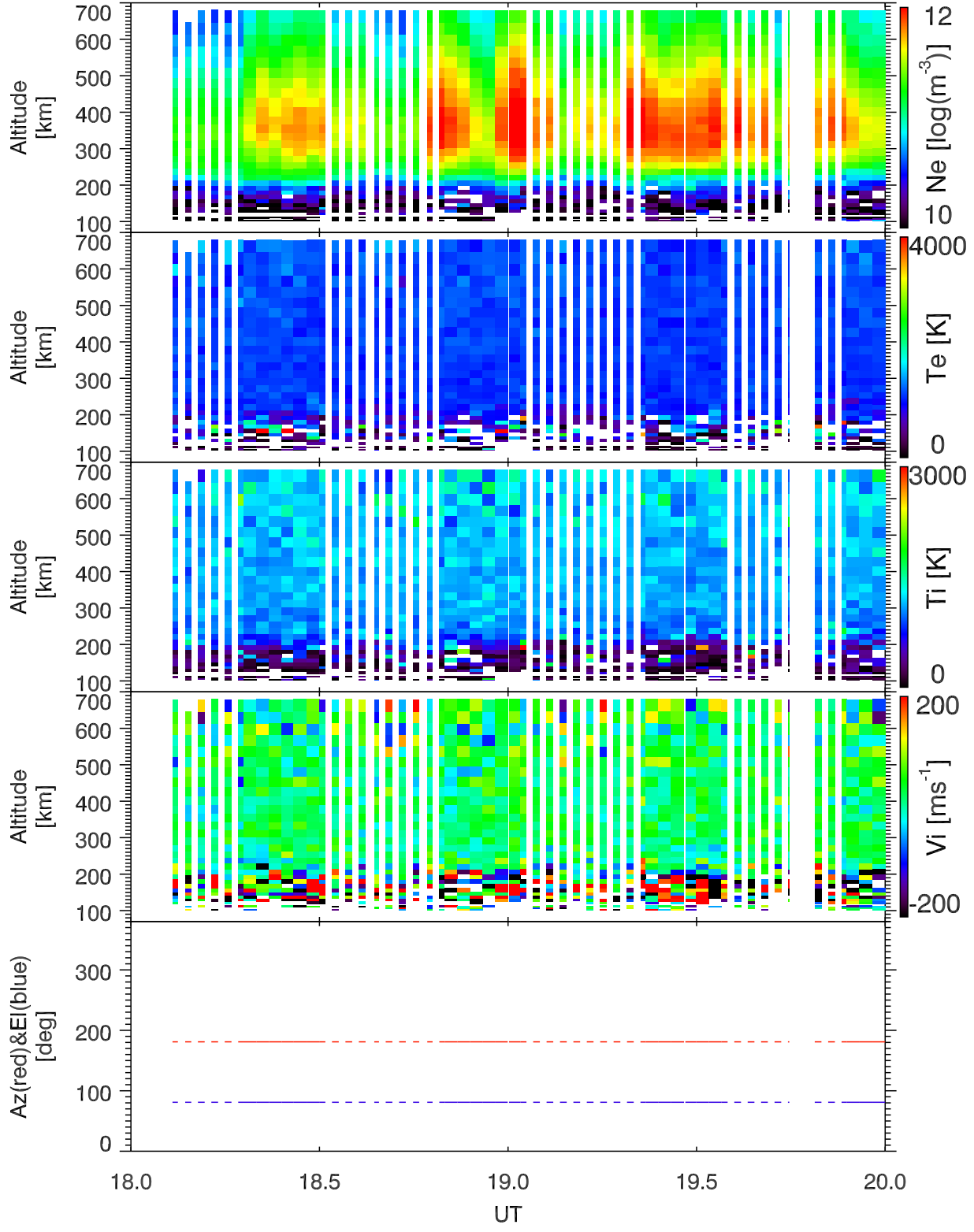
EISCAT 2001-12-11_18_20UT_tau0_120@42m.
