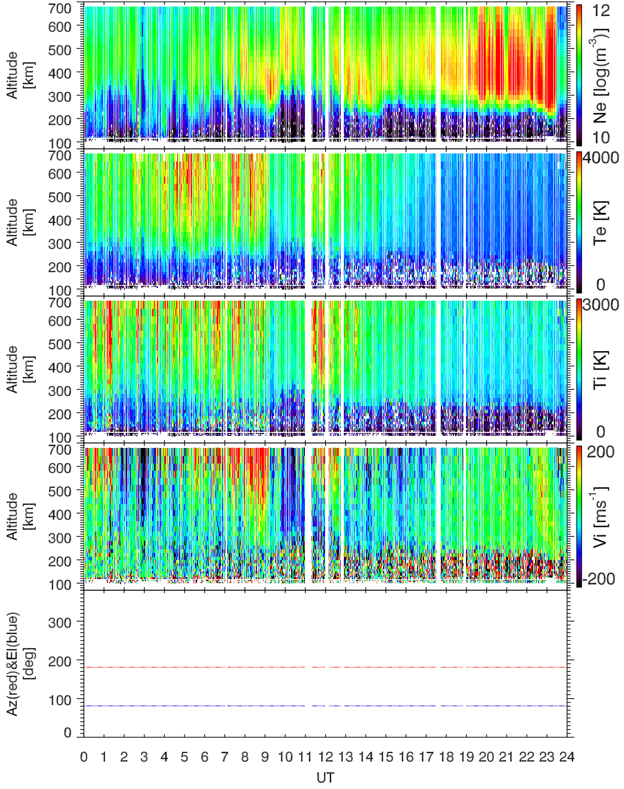
EISCAT 2001-12-12_00_24UT_tau0_120@42m.
