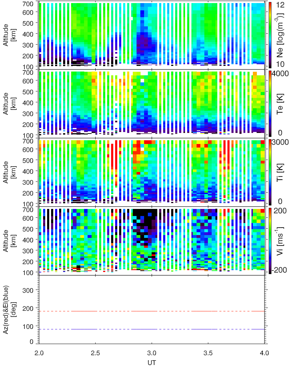
EISCAT 2001-12-12_02_04UT_tau0_120@42m.
