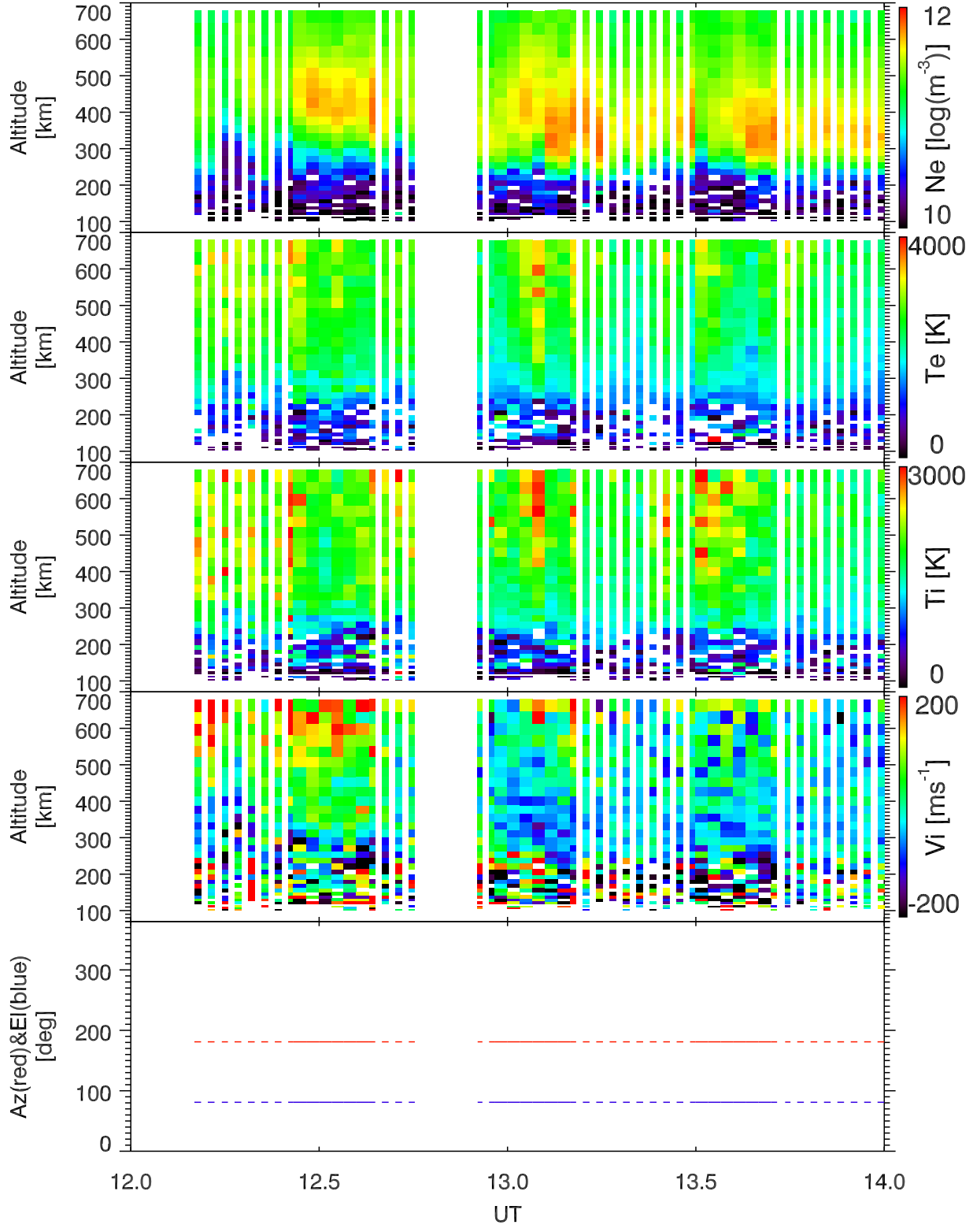
EISCAT 2001-12-12_12_14UT_tau0_120@42m.
