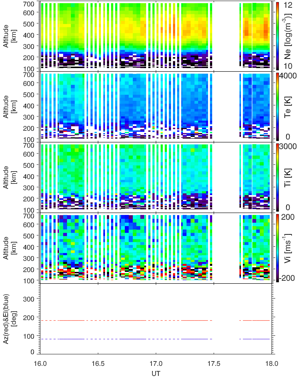
EISCAT 2001-12-12_16_18UT_tau0_120@42m.
