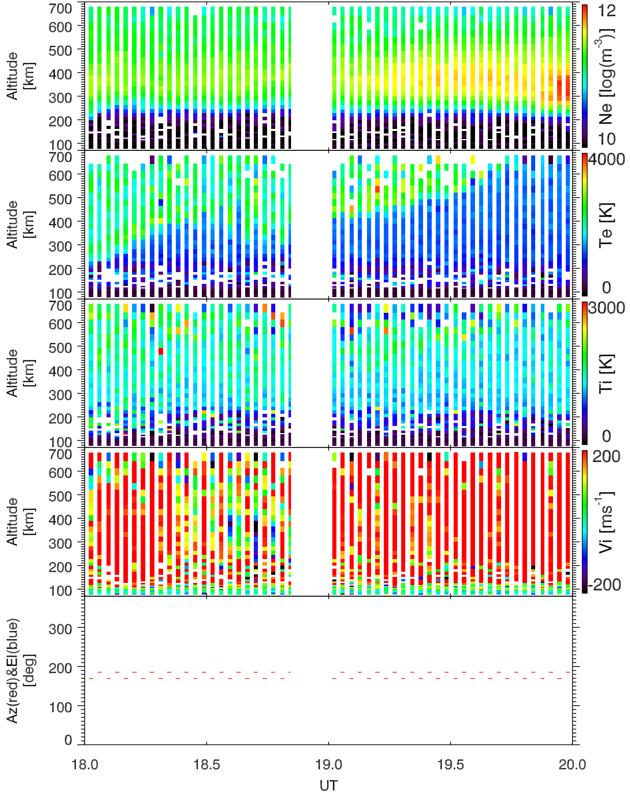
EISCAT 2001-12-12_18_20UT_tau0_ant@32m.
