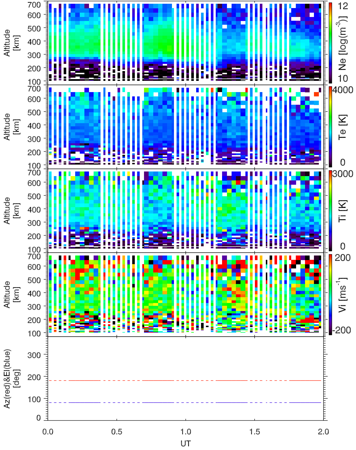
EISCAT 2001-12-13_00_02UT_tau0_120@42m.
