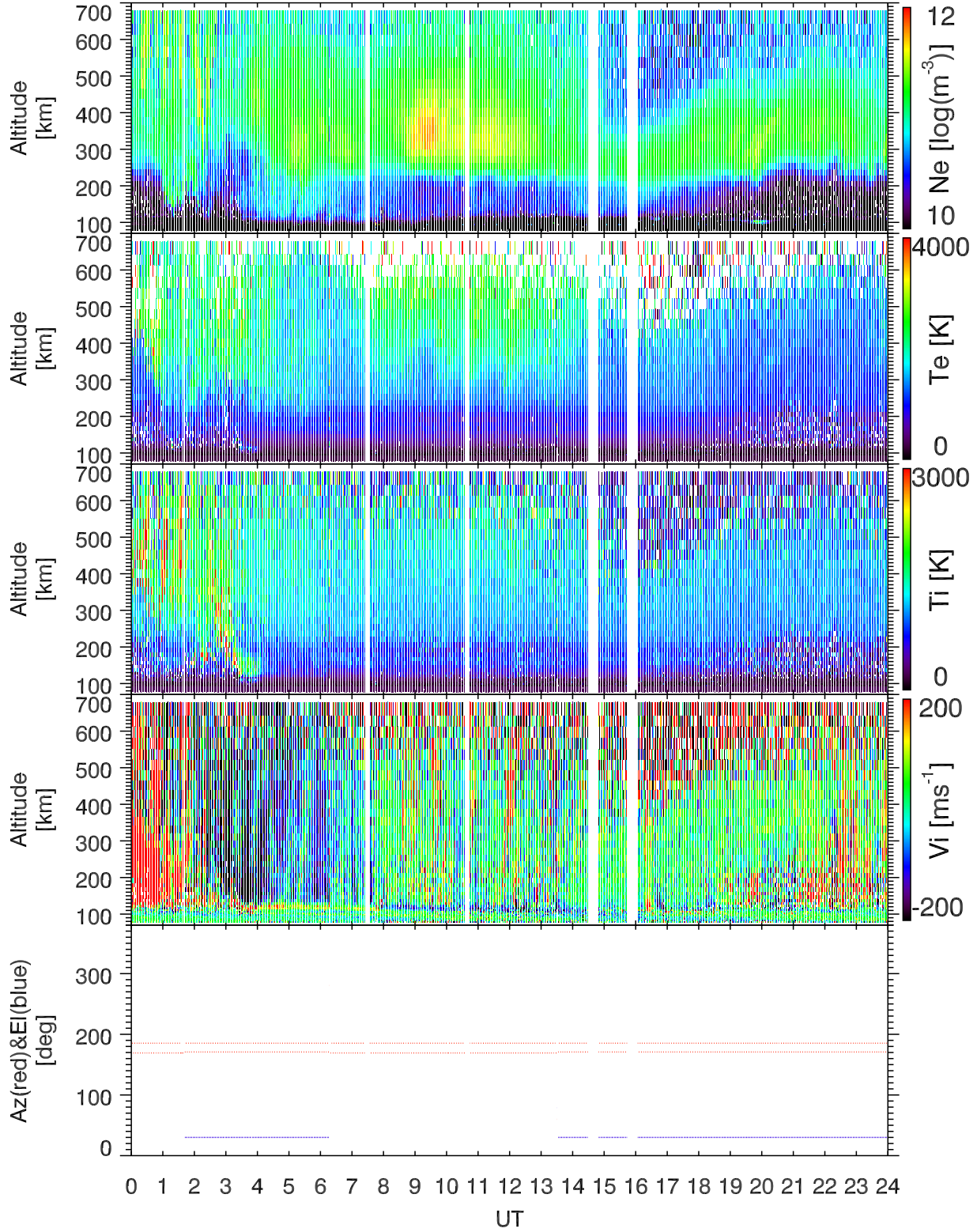
EISCAT 2001-12-13_00_24UT_tau0_ant@32m.
